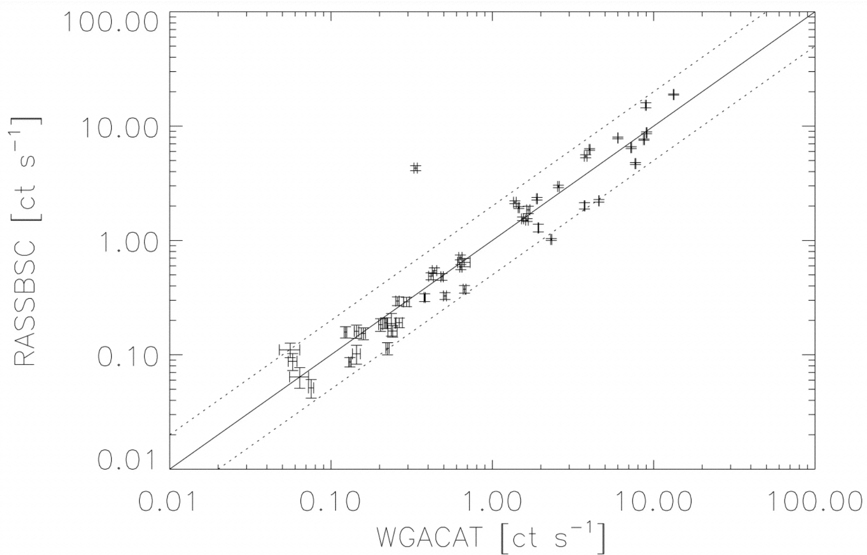
Fig. 3. from On XRay Variability in Active Binary Stars Kashyap & Drake 1999 ApJ 524 988 doi:10.1086/307821 https://dx.doi.org/10.1086/307821 © 1999. The American Astronomical Society. All rights reserved. Printed in U.S.A.
