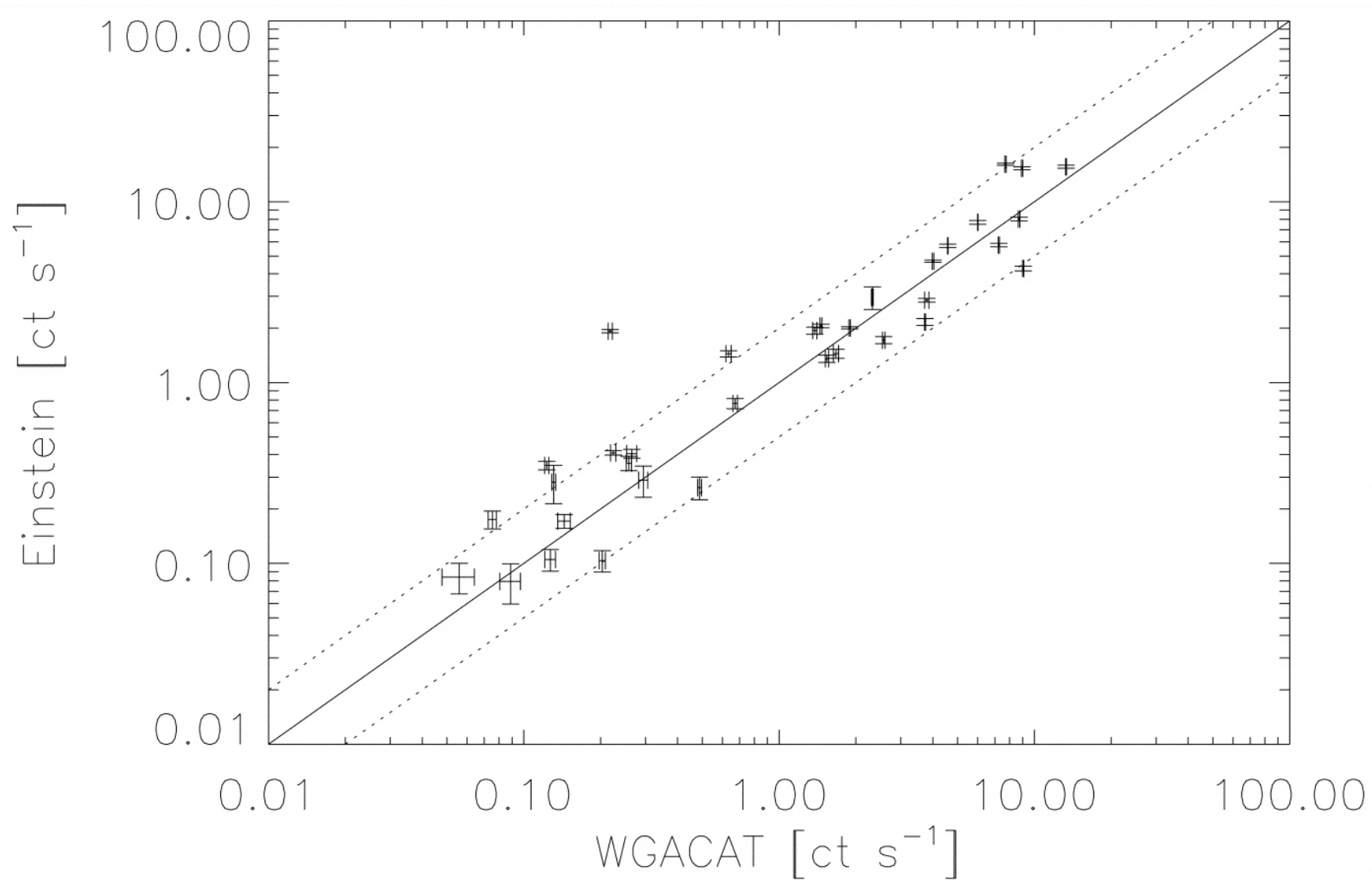
Fig. 2. from On XRay Variability in Active Binary Stars Kashyap & Drake 1999 ApJ 524 988 doi:10.1086/307821 https://dx.doi.org/10.1086/307821 © 1999. The American Astronomical Society. All rights reserved. Printed in U.S.A.
