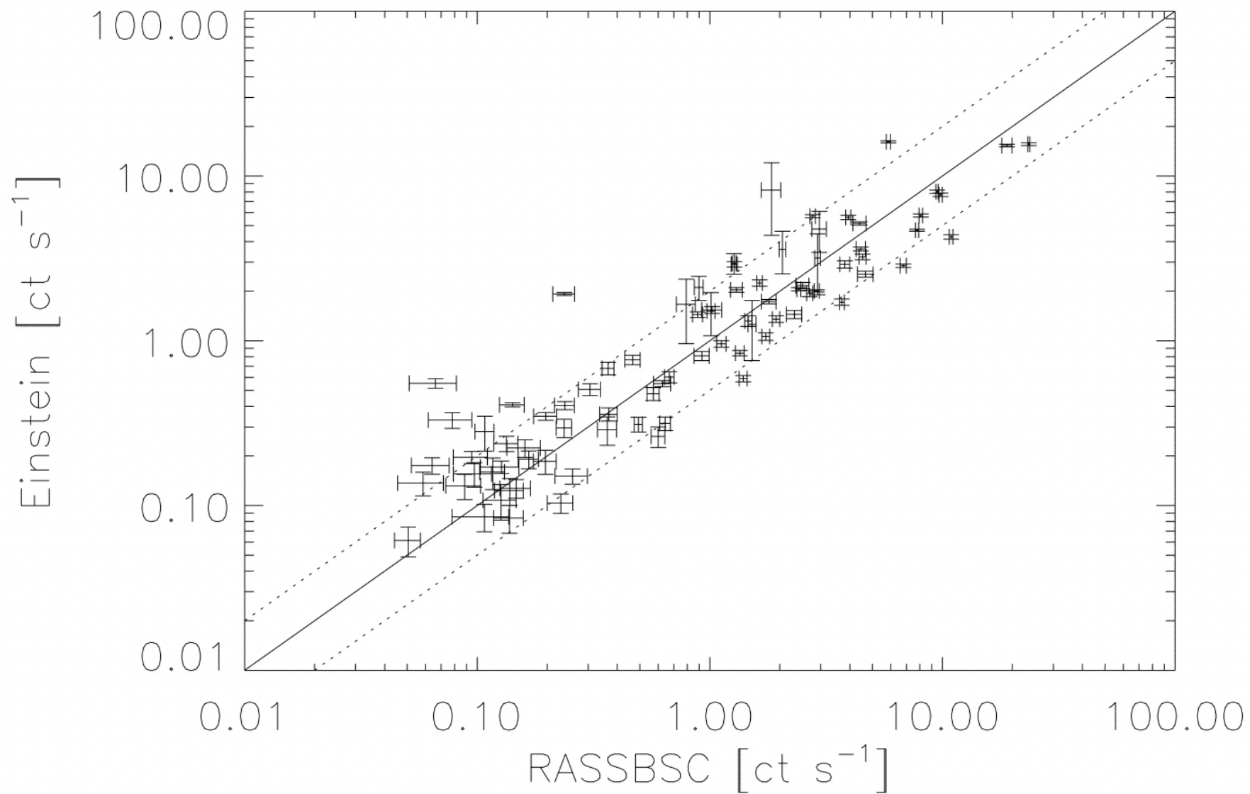
Fig. 1. from On XRay Variability in Active Binary Stars Kashyap & Drake 1999 ApJ 524 988 doi:10.1086/307821 https://dx.doi.org/10.1086/307821 © 1999. The American Astronomical Society. All rights reserved. Printed in U.S.A.
