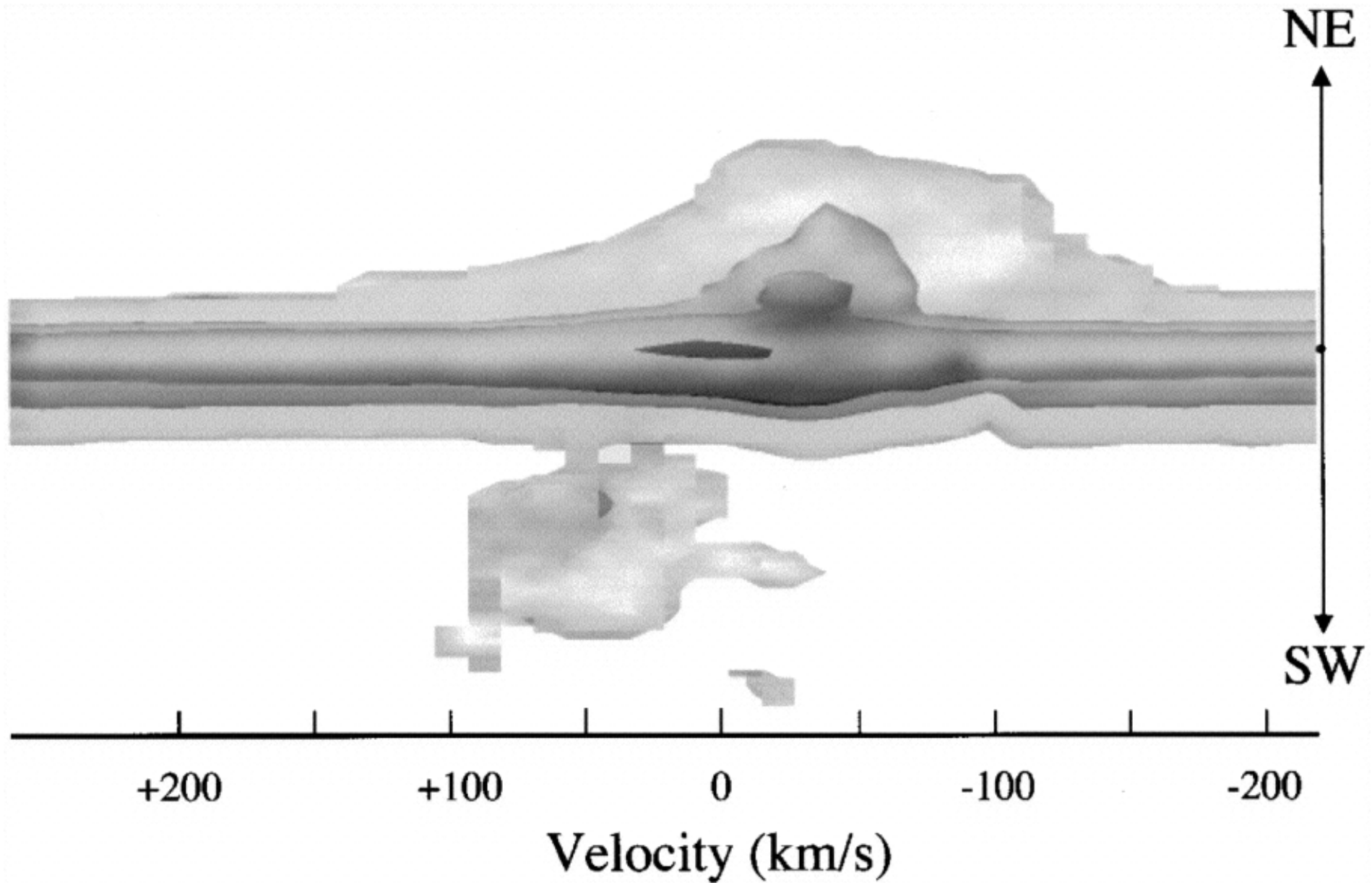
Fig. 4. from The [N II] Kinematics of R Aquarii Hollis et al. 1999 ApJ 522 297 doi:10.1086/307631 https://dx.doi.org/10.1086/307631
