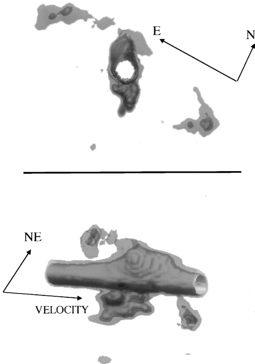
Fig. 3. from The [N II] Kinematics of R Aquarii Hollis et al. 1999 ApJ 522 297 doi:10.1086/307631 https://dx.doi.org/10.1086/307631
