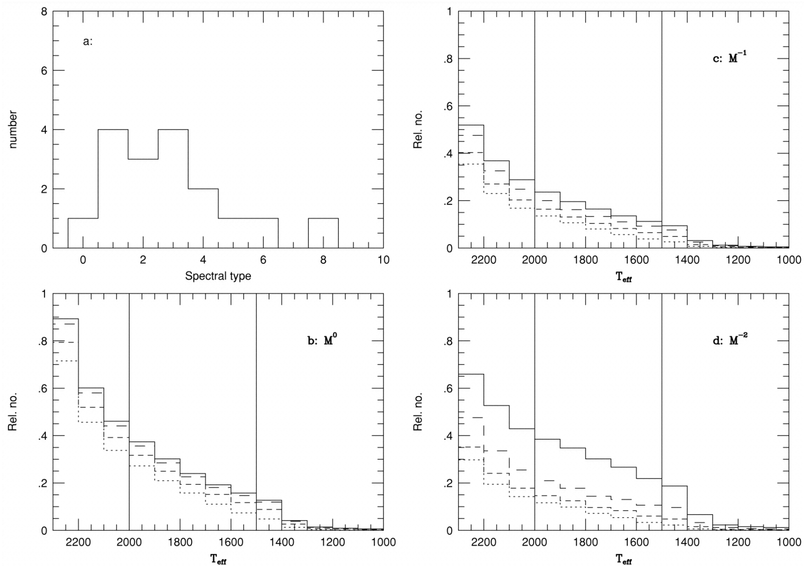
Fig. 8. from L Dwarfs and the Substellar Mass Function Reid et al. 1999 ApJ 521 613 doi:10.1086/307589 https://dx.doi.org/10.1086/307589 © 1999. The American Astronomical Society. All rights reserved. Printed in U.S.A.
