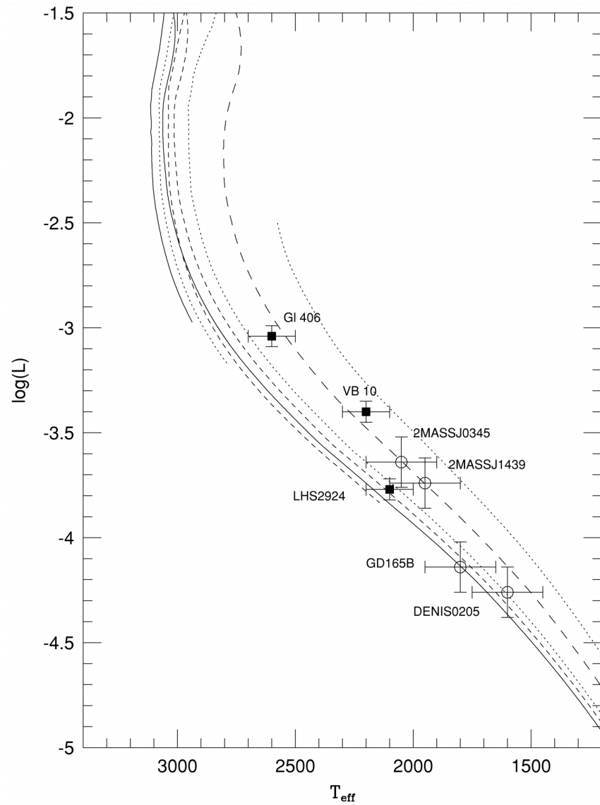
Fig. 7. from L Dwarfs and the Substellar Mass Function Reid et al. 1999 ApJ 521 613 doi:10.1086/307589 https://dx.doi.org/10.1086/307589 © 1999. The American Astronomical Society. All rights reserved. Printed in U.S.A.
