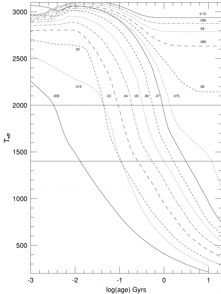
Fig. 6. from L Dwarfs and the Substellar Mass Function Reid et al. 1999 ApJ 521 613 doi:10.1086/307589 https://dx.doi.org/10.1086/307589 © 1999. The American Astronomical Society. All rights reserved. Printed in U.S.A.
