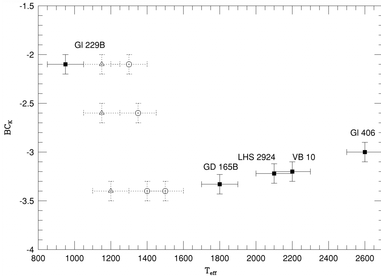
Fig. 5. from L Dwarfs and the Substellar Mass Function Reid et al. 1999 ApJ 521 613 doi:10.1086/307589 https://dx.doi.org/10.1086/307589 © 1999. The American Astronomical Society. All rights reserved. Printed in U.S.A.
