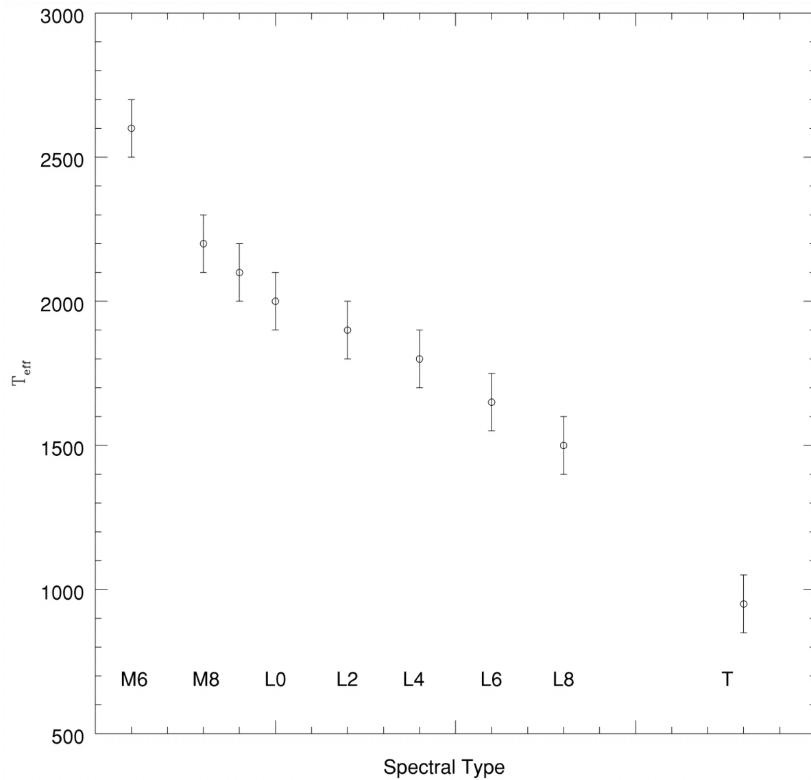
Fig. 4. from L Dwarfs and the Substellar Mass Function Reid et al. 1999 ApJ 521 613 doi:10.1086/307589 https://dx.doi.org/10.1086/307589 © 1999. The American Astronomical Society. All rights reserved. Printed in U.S.A.
