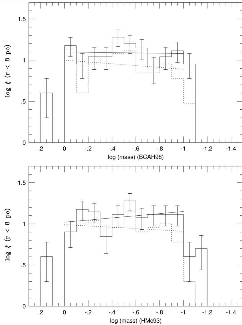
Fig. 2. from L Dwarfs and the Substellar Mass Function Reid et al. 1999 ApJ 521 613 doi:10.1086/307589 https://dx.doi.org/10.1086/307589 © 1999. The American Astronomical Society. All rights reserved. Printed in U.S.A.
