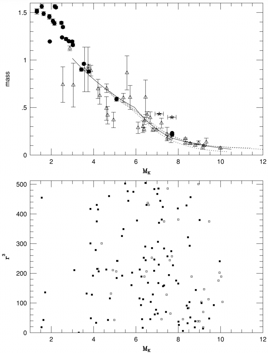
Fig. 1. from L Dwarfs and the Substellar Mass Function Reid et al. 1999 ApJ 521 613 doi:10.1086/307589 https://dx.doi.org/10.1086/307589 © 1999. The American Astronomical Society. All rights reserved. Printed in U.S.A.
