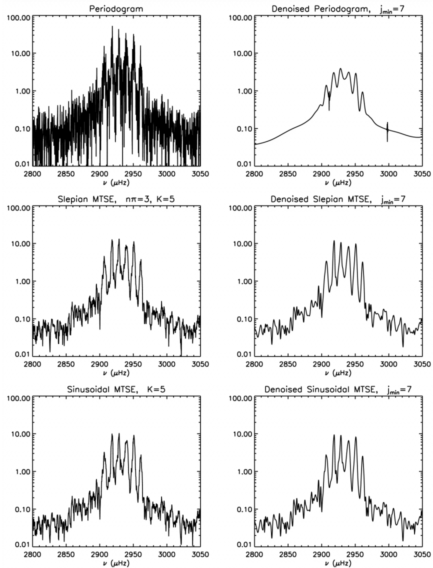
Fig. 4. from Multitaper Spectral Analysis and Wavelet Denoising Applied to Helioseismic Data Komm et al. 1999 ApJ 519 407 doi:10.1086/307359 https://dx.doi.org/10.1086/307359 © 1999. The American Astronomical Society. All rights reserved. Printed in U.S.A.
