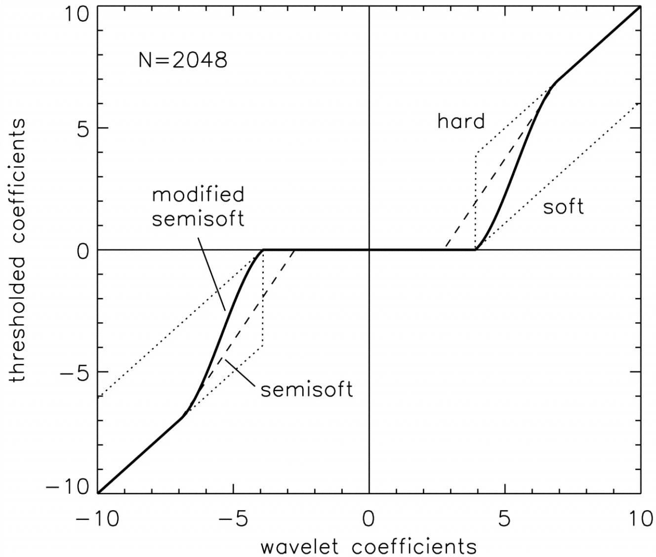
Fig. 3. from Multitaper Spectral Analysis and Wavelet Denoising Applied to Helioseismic Data Komm et al. 1999 ApJ 519 407 doi:10.1086/307359 https://dx.doi.org/10.1086/307359 © 1999. The American Astronomical Society. All rights reserved. Printed in U.S.A.
