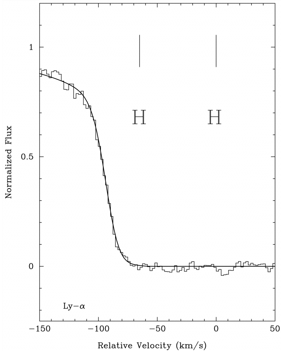
Fig. 2. from Deuterium toward Quasar Q0014+813 Burles, Kirkman, & Tytler 1999 ApJ 519 18 doi:10.1086/307331 https://dx.doi.org/10.1086/307331 © 1999. The American Astronomical Society. All rights reserved. Printed in U.S.A.
