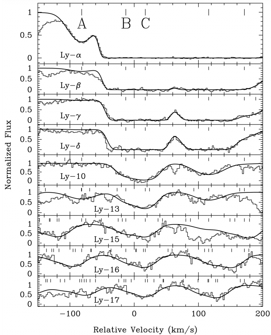
Fig. 1. from Deuterium toward Quasar Q0014+813 Burles, Kirkman, & Tytler 1999 ApJ 519 18 doi:10.1086/307331 https://dx.doi.org/10.1086/307331 © 1999. The American Astronomical Society. All rights reserved. Printed in U.S.A.
