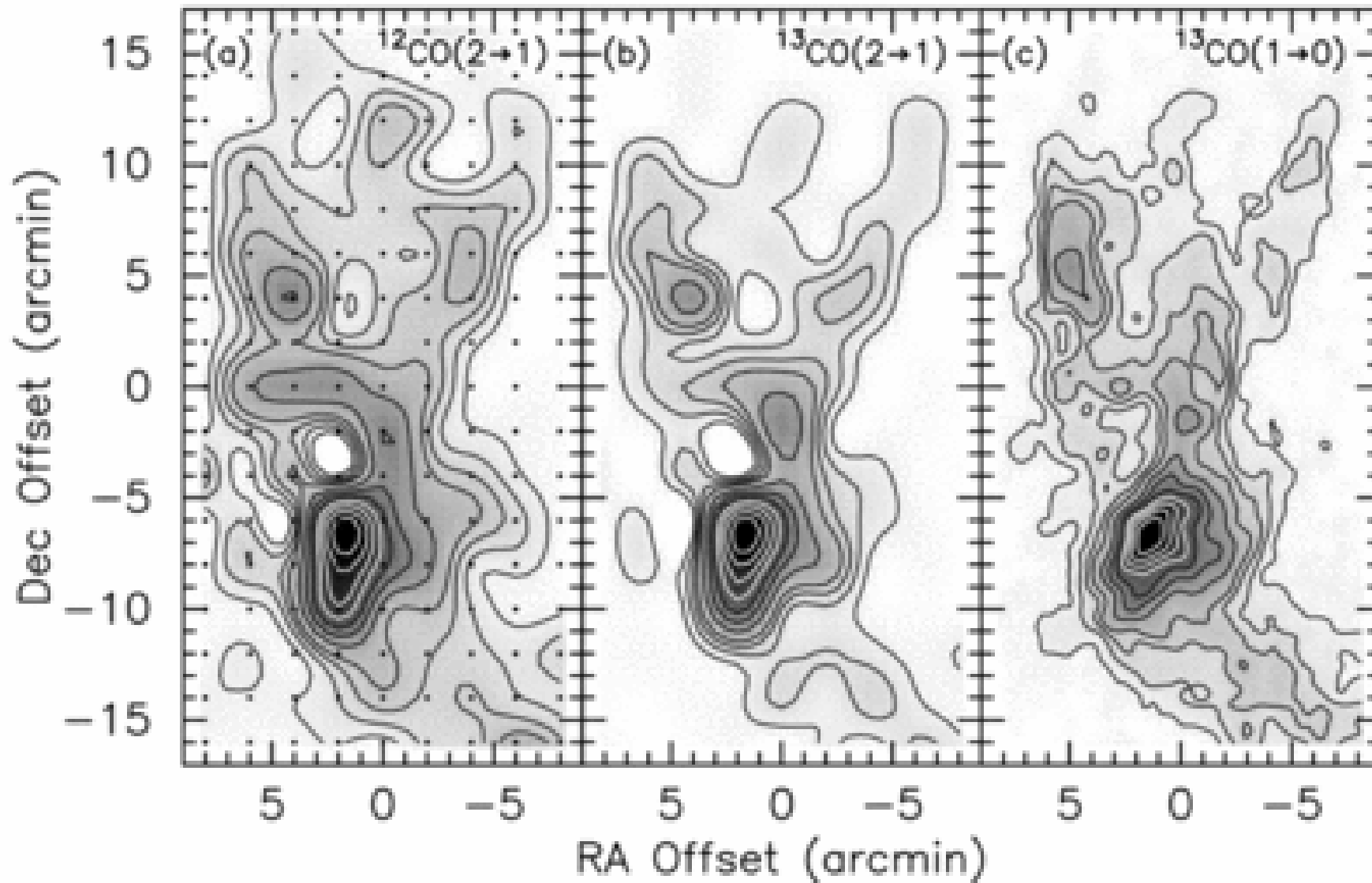
Fig. 1. from The LargeScale J=32 and J=21 CO Emission from M17 and Its Implications for Extragalactic CO Observations Wilson, Howe, & Balogh 1999 ApJ 517 174 doi:10.1086/307180 https://dx.doi.org/10.1086/307180 © 1999. The American Astronomical Society. All rights reserved. Printed in U.S.A.
