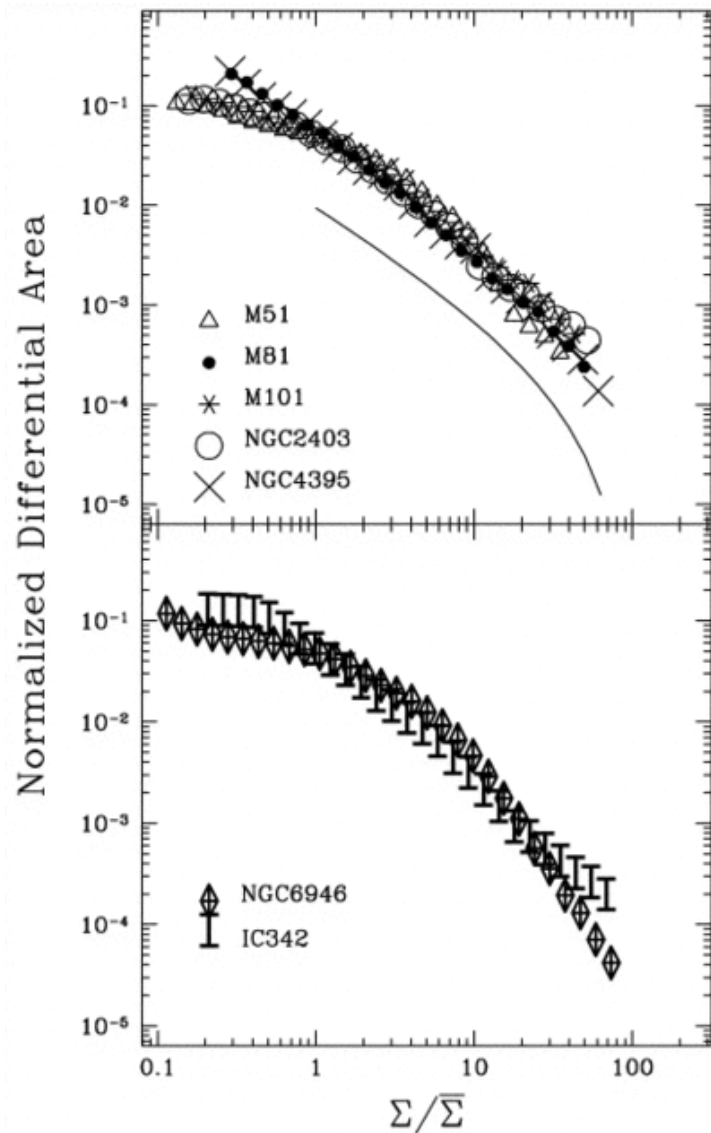
Fig. 3. from On the Structure and Morphology of the “Diffuse Ionized Medium” in Starforming Galaxies Wang, Heckman, & Lehnert 1999 ApJ 515 97 doi:10.1086/307008 https://dx.doi.org/10.1086/307008 © 1999. The American Astronomical Society. All rights reserved. Printed in U.S.A.
