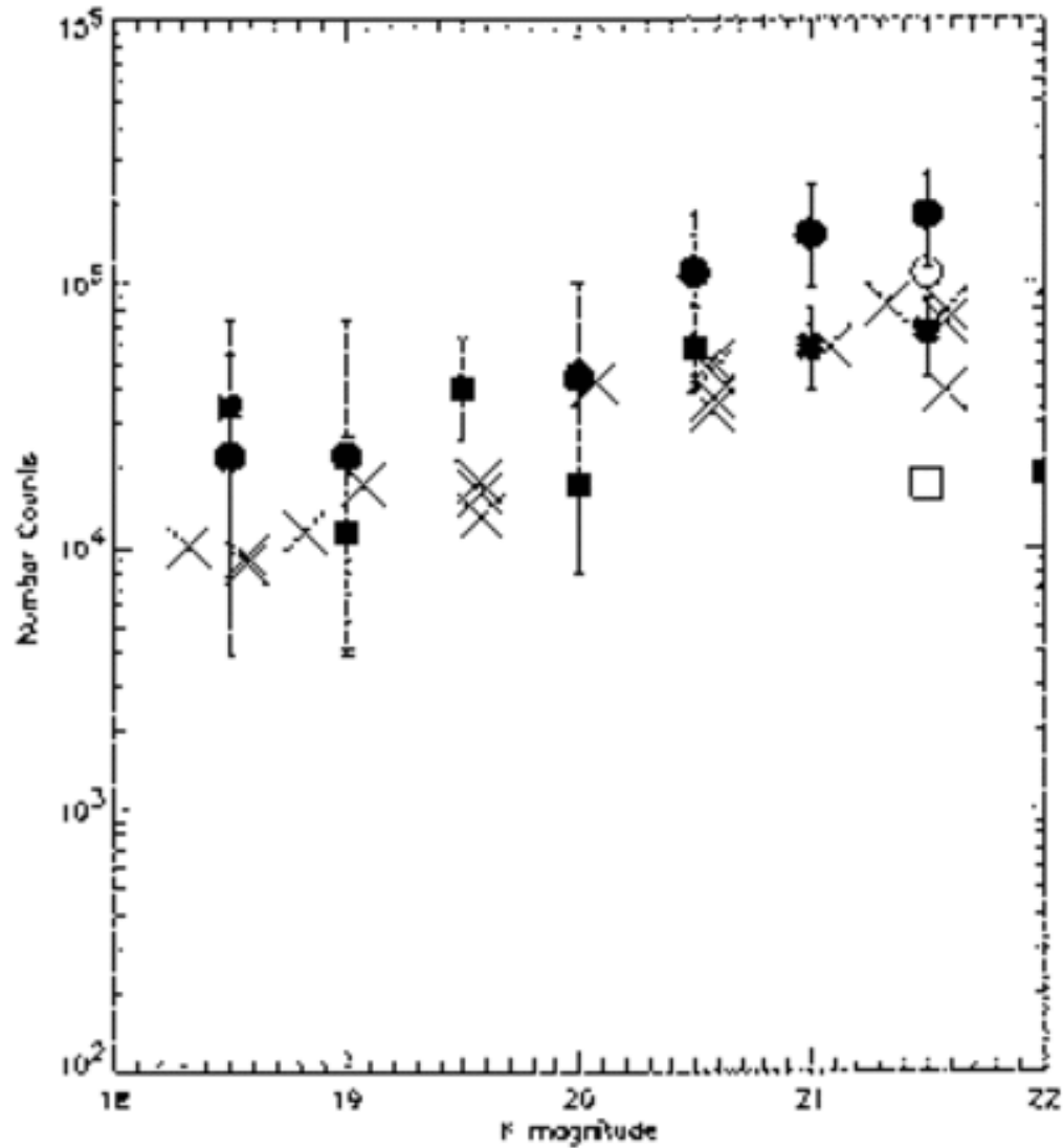
Fig. 4. from A Narrowband Imaging Search for [O III] Emission from Galaxies at z > 3 Teplitz, Malkan, & McLean 1999 ApJ 514 33 doi:10.1086/306947 https://dx.doi.org/10.1086/306947 © 1999. The American Astronomical Society. All rights reserved. Printed in U.S.A.
