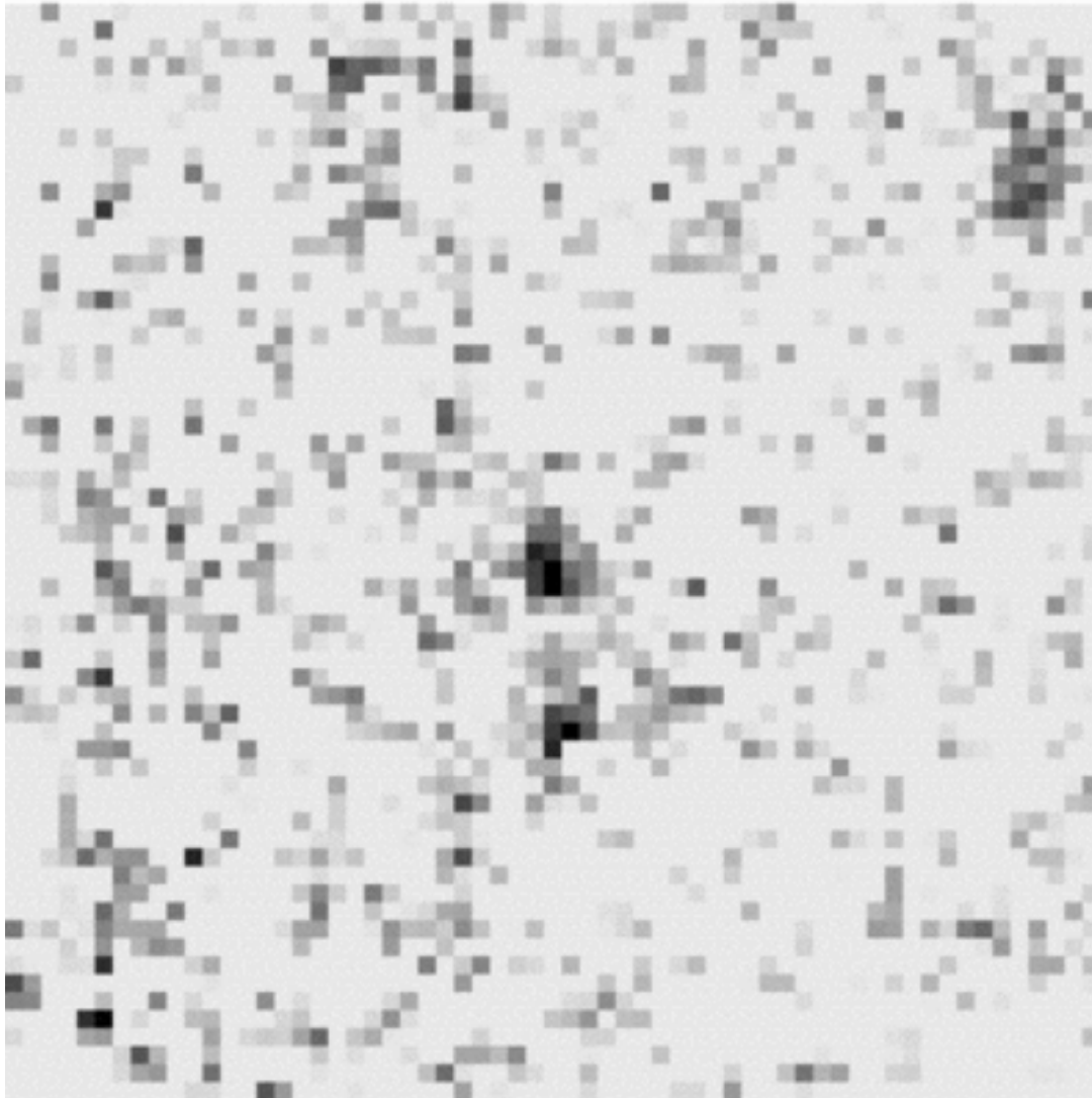
Fig. 3. from A Narrowband Imaging Search for [O III] Emission from Galaxies at z > 3 Teplitz, Malkan, & McLean 1999 ApJ 514 33 doi:10.1086/306947 https://dx.doi.org/10.1086/306947 © 1999. The American Astronomical Society. All rights reserved. Printed in U.S.A.
