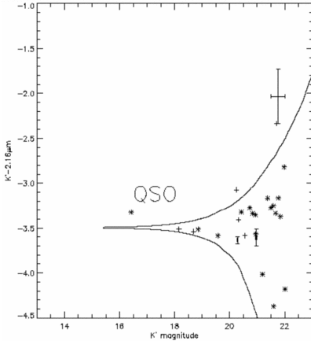
Fig. 2. from A Narrowband Imaging Search for [O III] Emission from Galaxies at z > 3 Teplitz, Malkan, & McLean 1999 ApJ 514 33 doi:10.1086/306947 https://dx.doi.org/10.1086/306947 © 1999. The American Astronomical Society. All rights reserved. Printed in U.S.A.
