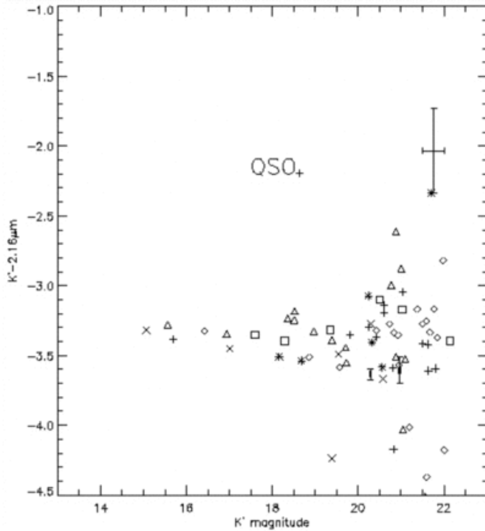
Fig. 1. from A Narrowband Imaging Search for [O III] Emission from Galaxies at z > 3 Teplitz, Malkan, & McLean 1999 ApJ 514 33 doi:10.1086/306947 https://dx.doi.org/10.1086/306947 © 1999. The American Astronomical Society. All rights reserved. Printed in U.S.A.
