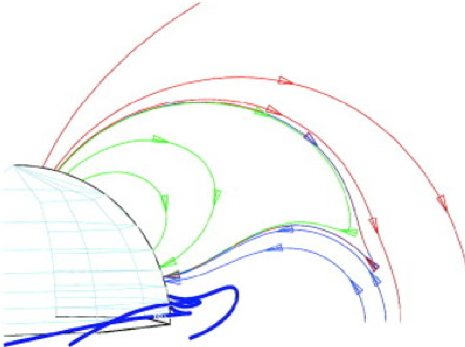
Fig. 4. from A Model for Solar Coronal Mass Ejections Antiochos, DeVore, & Klimchuk 1999 ApJ 510 485 doi:10.1086/306563 https://dx.doi.org/10.1086/306563 No copyright is claimed for this article. Printed in U.S.A.
