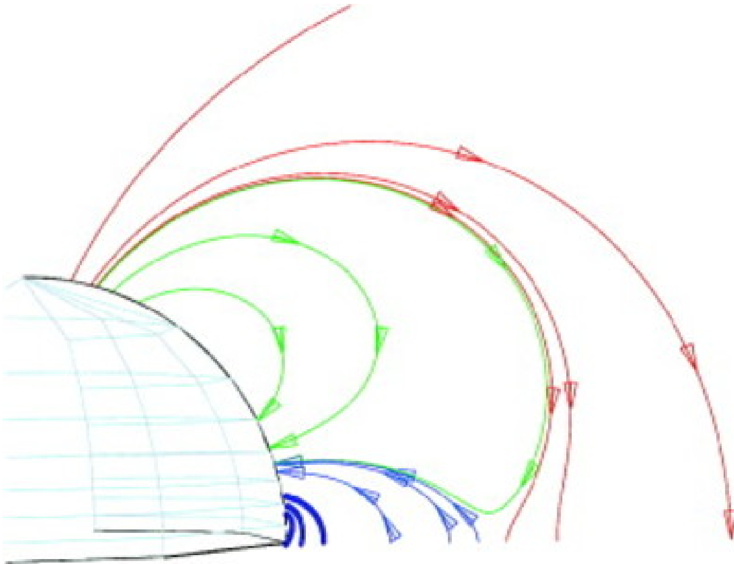
Fig. 4. from A Model for Solar Coronal Mass Ejections Antiochos, DeVore, & Klimchuk 1999 ApJ 510 485 doi:10.1086/306563 https://dx.doi.org/10.1086/306563 No copyright is claimed for this article. Printed in U.S.A.
