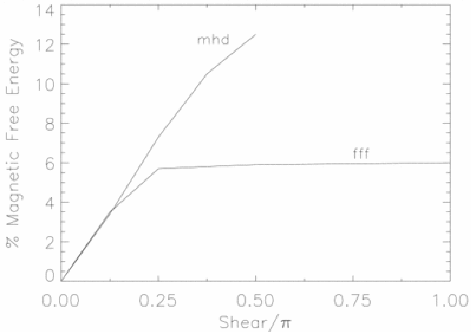
Fig. 3. from A Model for Solar Coronal Mass Ejections Antiochos, DeVore, & Klimchuk 1999 ApJ 510 485 doi:10.1086/306563 https://dx.doi.org/10.1086/306563 No copyright is claimed for this article. Printed in U.S.A.
