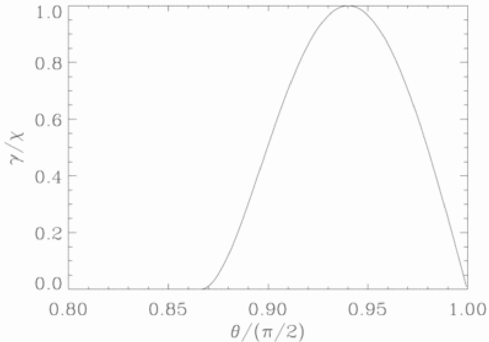
Fig. 2. from A Model for Solar Coronal Mass Ejections Antiochos, DeVore, & Klimchuk 1999 ApJ 510 485 doi:10.1086/306563 https://dx.doi.org/10.1086/306563 No copyright is claimed for this article. Printed in U.S.A.
