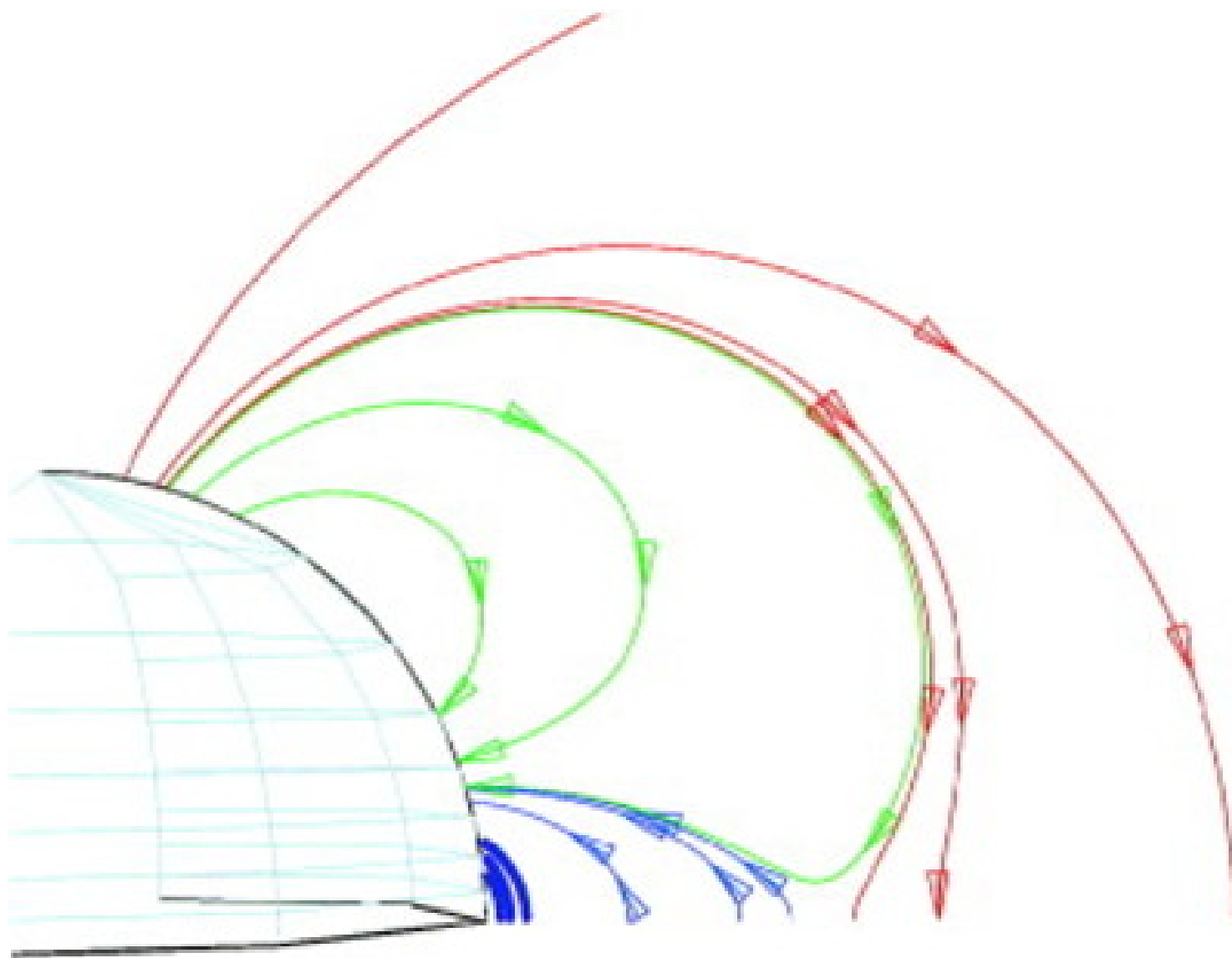
Fig. 1. from A Model for Solar Coronal Mass Ejections Antiochos, DeVore, & Klimchuk 1999 ApJ 510 485 doi:10.1086/306563 https://dx.doi.org/10.1086/306563 No copyright is claimed for this article. Printed in U.S.A.
