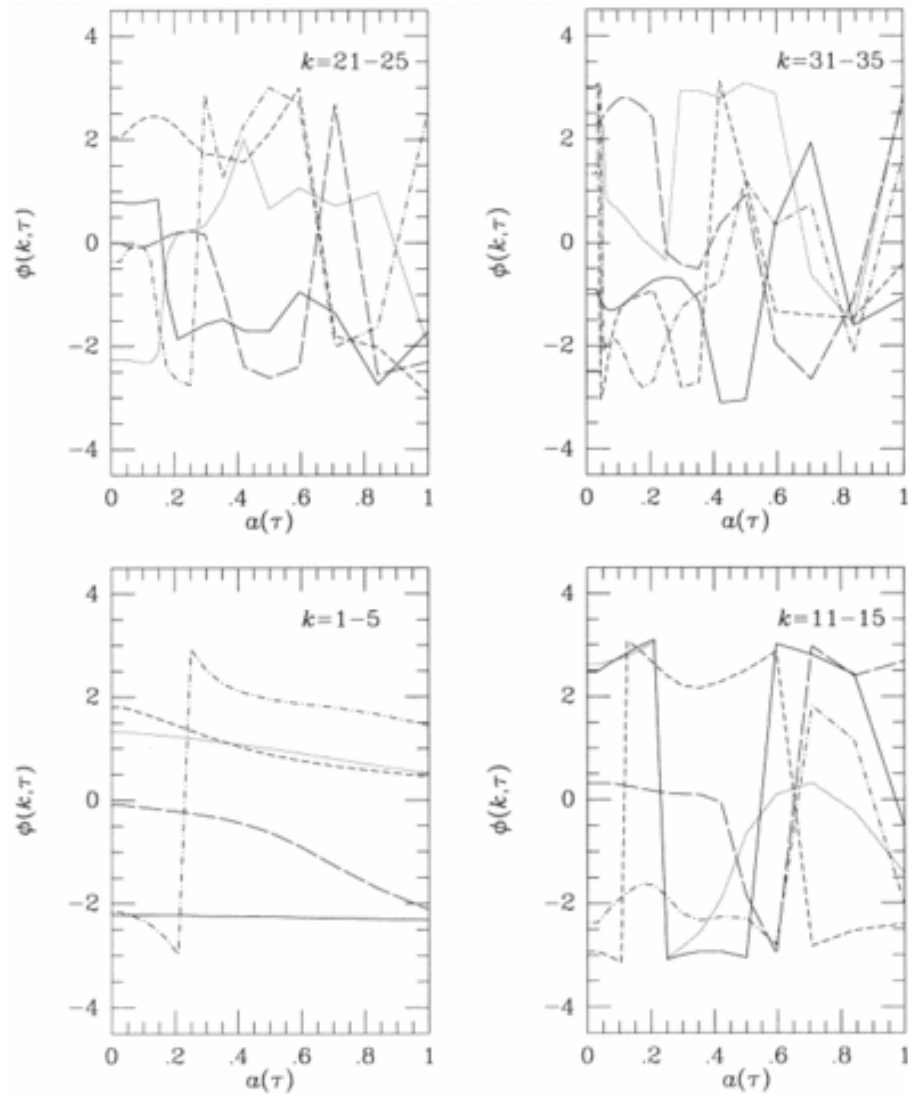
Fig. 8. from SelfSimilar Evolution of Gravitational Clustering. II. NBody Simulations of the n = 2 Spectrum Jain & Bertschinger 1998 ApJ 509 517 doi:10.1086/306538 https://dx.doi.org/10.1086/306538 © 1998. The American Astronomical Society. All rights reserved. Printed in U.S.A.
