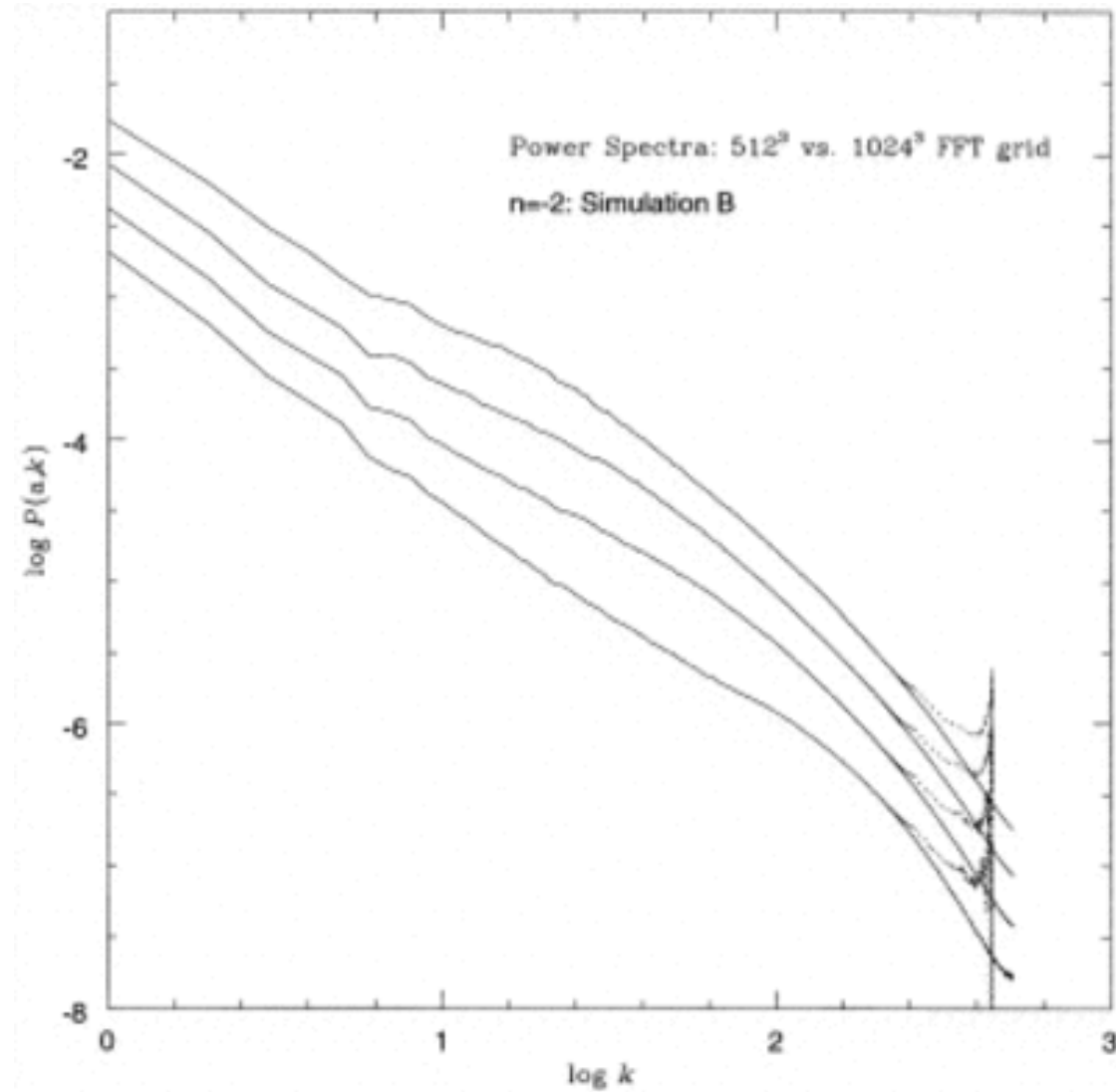
Fig. 2. from SelfSimilar Evolution of Gravitational Clustering. II. NBody Simulations of the n = 2 Spectrum Jain & Bertschinger 1998 ApJ 509 517 doi:10.1086/306538 https://dx.doi.org/10.1086/306538 © 1998. The American Astronomical Society. All rights reserved. Printed in U.S.A.
