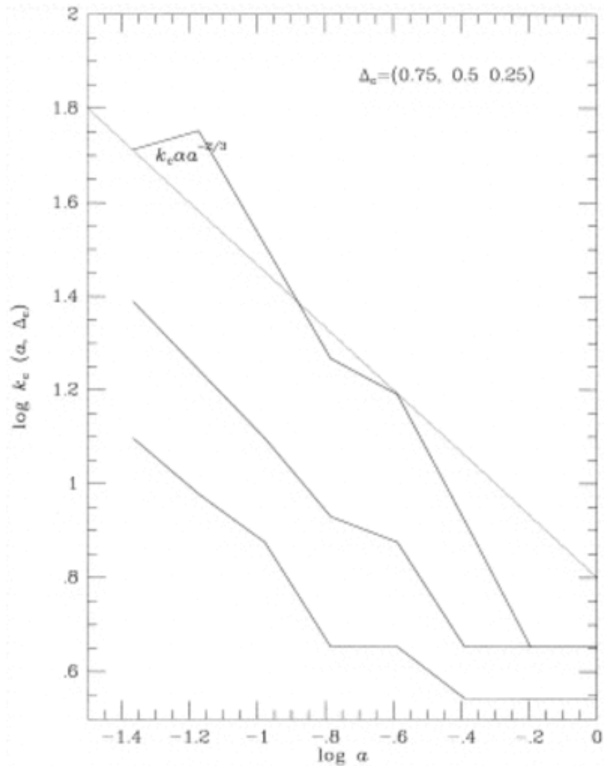
Fig. 14. from SelfSimilar Evolution of Gravitational Clustering. II. NBody Simulations of the n = 2 Spectrum Jain & Bertschinger 1998 ApJ 509 517 doi:10.1086/306538 https://dx.doi.org/10.1086/306538 © 1998. The American Astronomical Society. All rights reserved. Printed in U.S.A.
