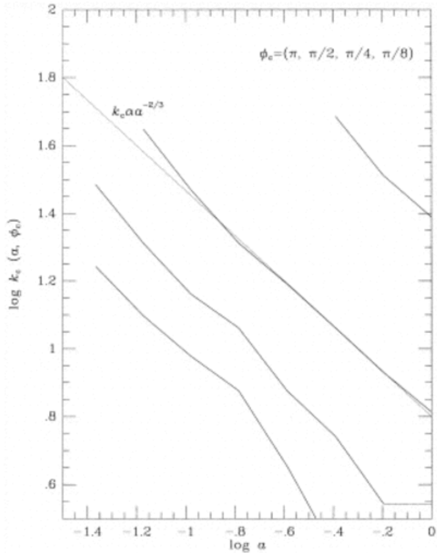
Fig. 13. from SelfSimilar Evolution of Gravitational Clustering. II. NBody Simulations of the n = 2 Spectrum Jain & Bertschinger 1998 ApJ 509 517 doi:10.1086/306538 https://dx.doi.org/10.1086/306538 © 1998. The American Astronomical Society. All rights reserved. Printed in U.S.A.
