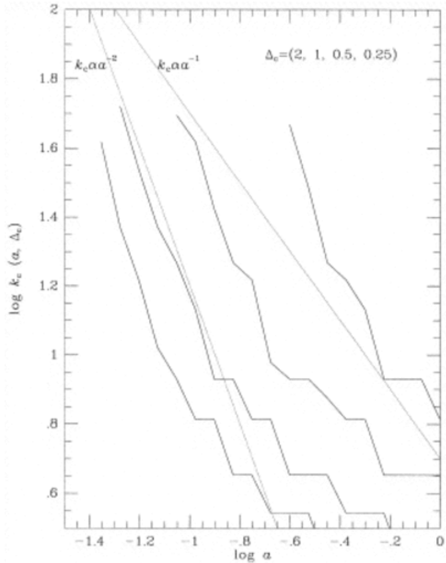
Fig. 12. from SelfSimilar Evolution of Gravitational Clustering. II. NBody Simulations of the n = 2 Spectrum Jain & Bertschinger 1998 ApJ 509 517 doi:10.1086/306538 https://dx.doi.org/10.1086/306538 © 1998. The American Astronomical Society. All rights reserved. Printed in U.S.A.
