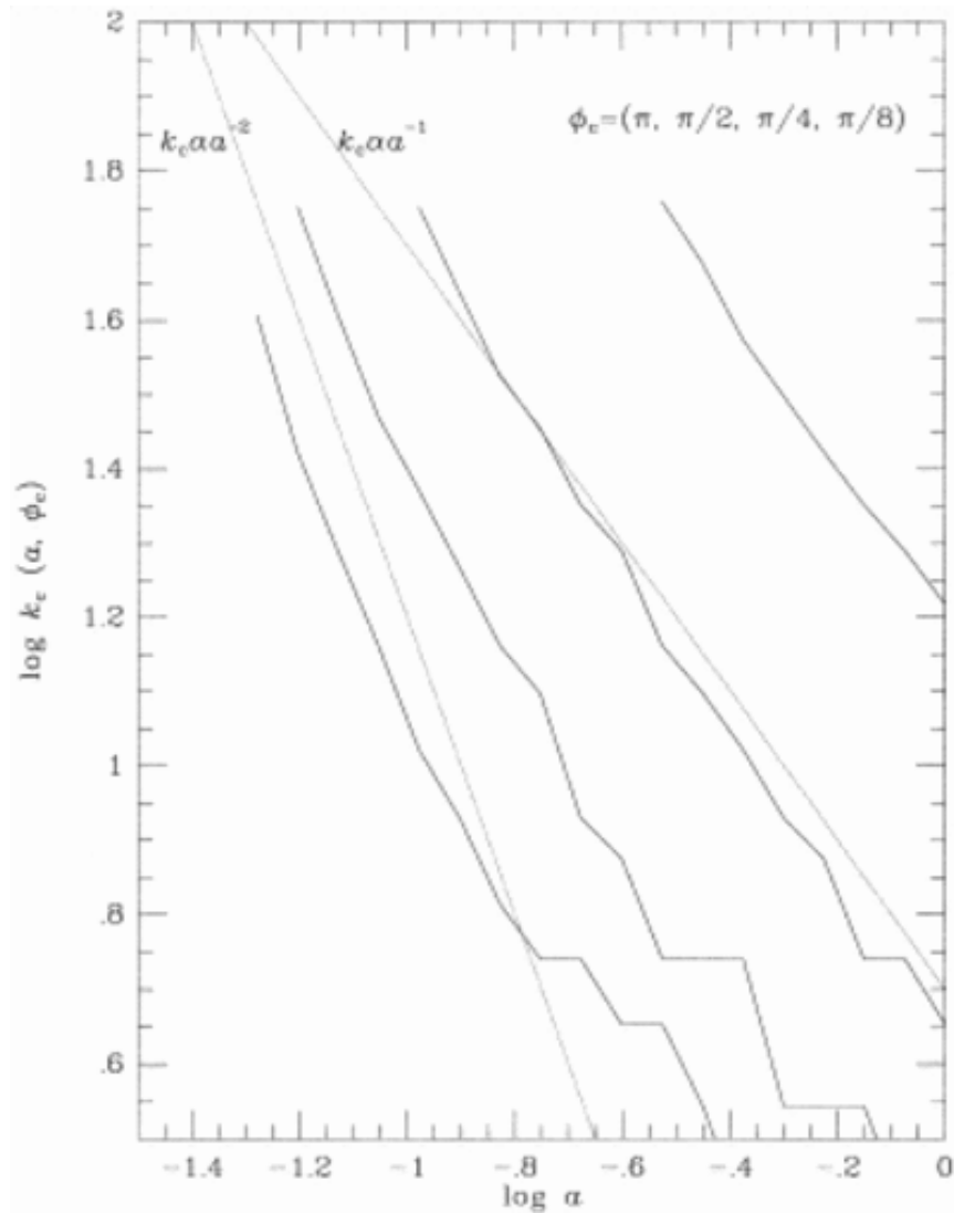
Fig. 11. from SelfSimilar Evolution of Gravitational Clustering. II. NBody Simulations of the n = 2 Spectrum Jain & Bertschinger 1998 ApJ 509 517 doi:10.1086/306538 https://dx.doi.org/10.1086/306538 © 1998. The American Astronomical Society. All rights reserved. Printed in U.S.A.
