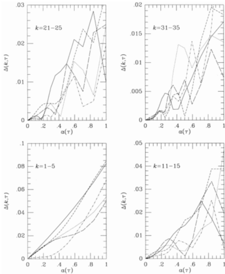
Fig. 10. from SelfSimilar Evolution of Gravitational Clustering. II. NBody Simulations of the n = 2 Spectrum Jain & Bertschinger 1998 ApJ 509 517 doi:10.1086/306538 https://dx.doi.org/10.1086/306538 © 1998. The American Astronomical Society. All rights reserved. Printed in U.S.A.
