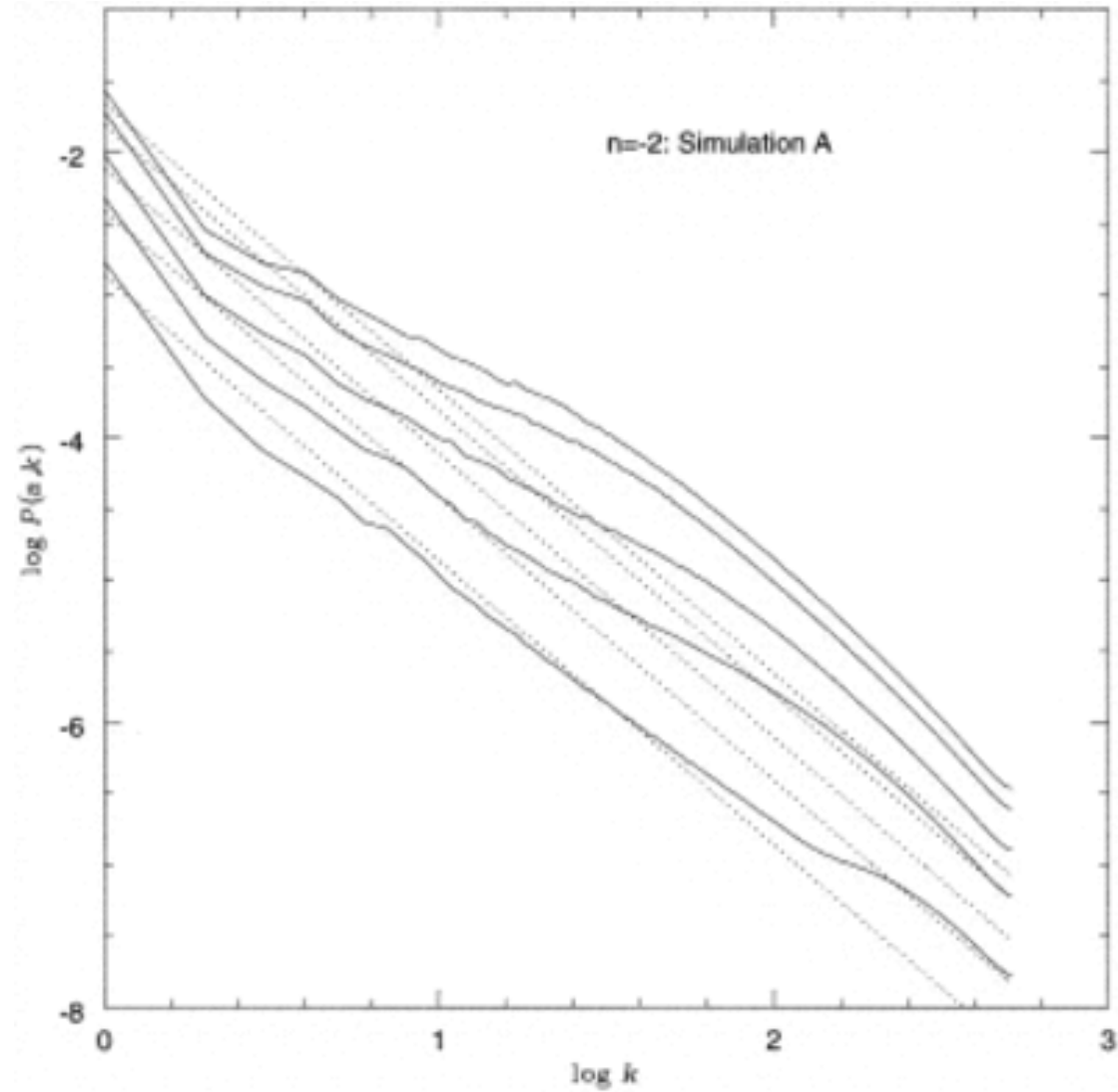
Fig. 1. from SelfSimilar Evolution of Gravitational Clustering. II. NBody Simulations of the n = 2 Spectrum Jain & Bertschinger 1998 ApJ 509 517 doi:10.1086/306538 https://dx.doi.org/10.1086/306538 © 1998. The American Astronomical Society. All rights reserved. Printed in U.S.A.
