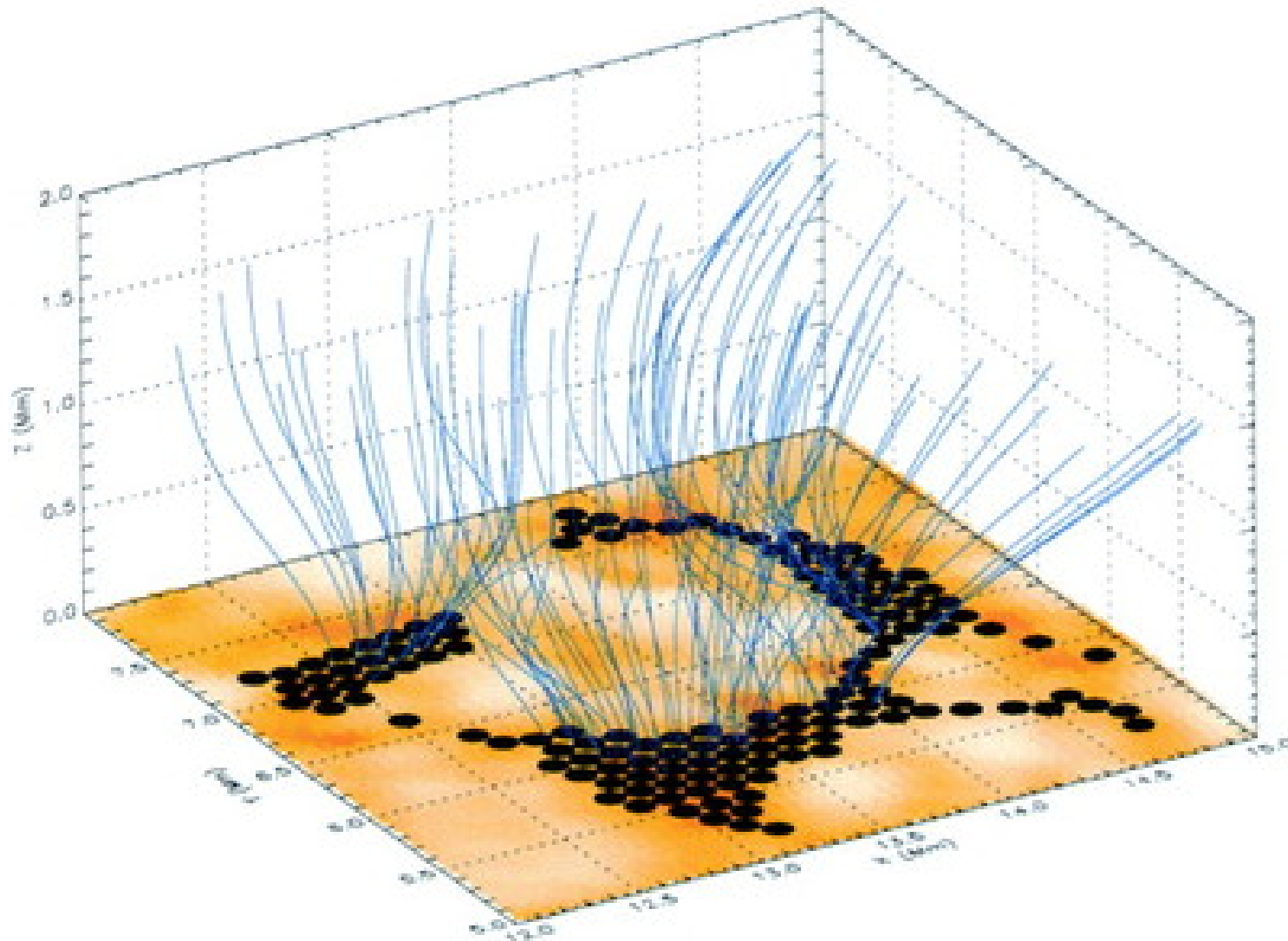
Fig. 9. from Dynamics of Magnetic Flux Elements in the Solar Photosphere van Ballegoijen et al. 1998 ApJ 509 435 doi:10.1086/306471 https://dx.doi.org/10.1086/306471 © 1998. The American Astronomical Society. All rights reserved. Printed in U.S.A.
