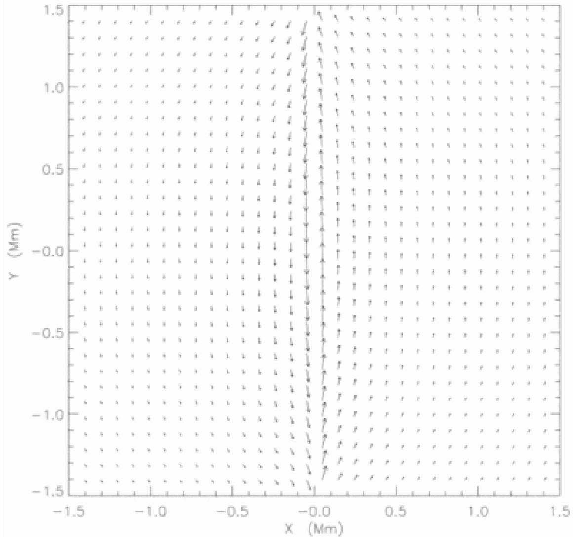
Fig. 8. from Dynamics of Magnetic Flux Elements in the Solar Photosphere van Ballegoijen et al. 1998 ApJ 509 435 doi:10.1086/306471 https://dx.doi.org/10.1086/306471 © 1998. The American Astronomical Society. All rights reserved. Printed in U.S.A.
