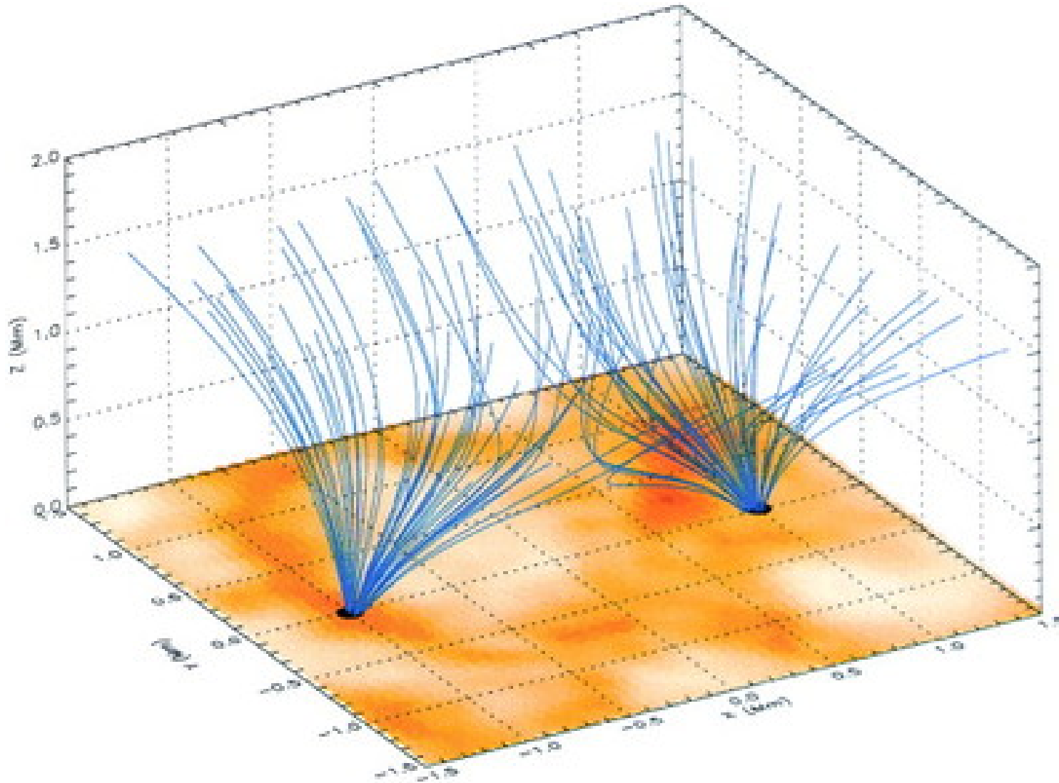
Fig. 7. from Dynamics of Magnetic Flux Elements in the Solar Photosphere van Ballegoijen et al. 1998 ApJ 509 435 doi:10.1086/306471 https://dx.doi.org/10.1086/306471 © 1998. The American Astronomical Society. All rights reserved. Printed in U.S.A.
