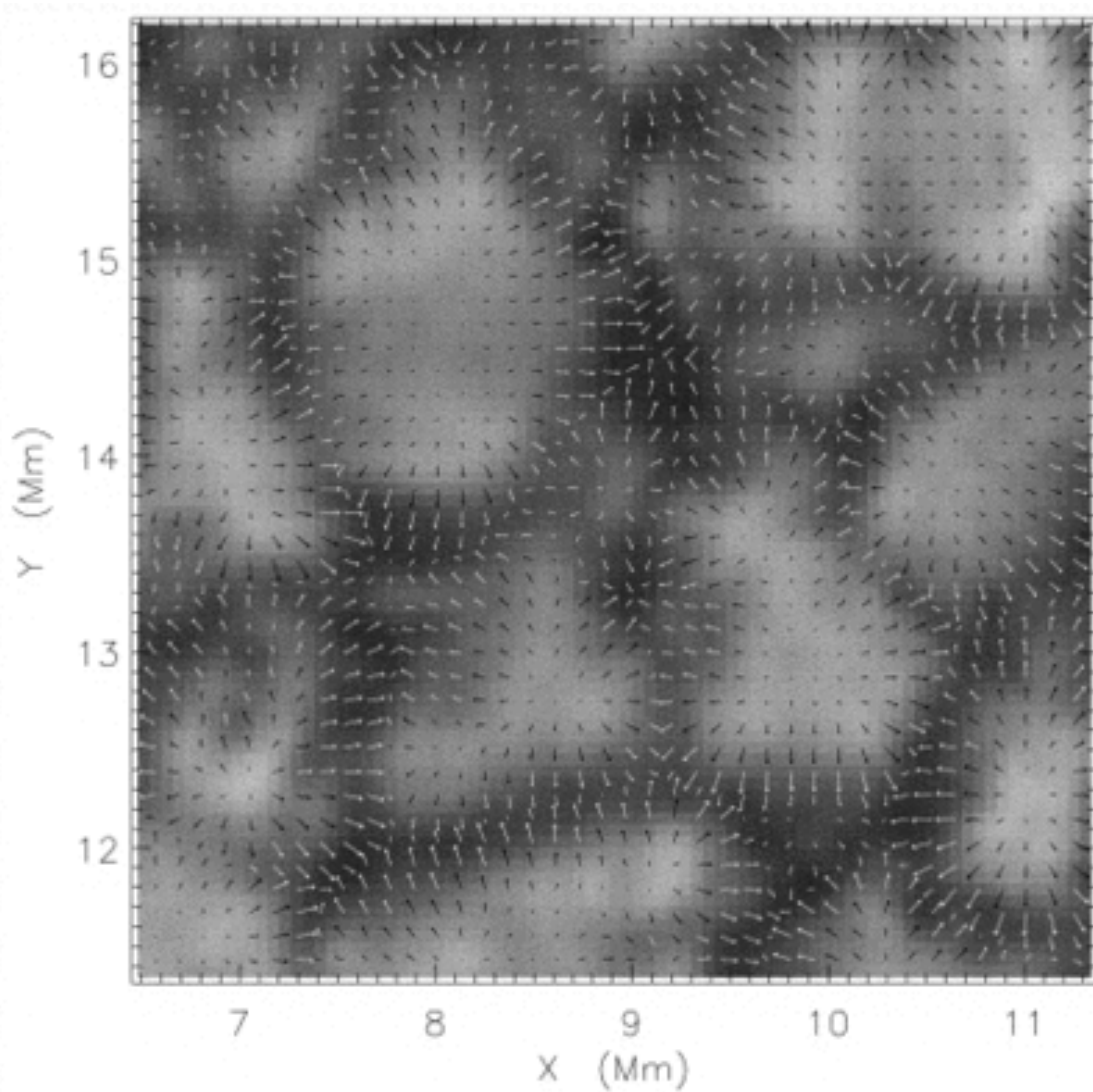
Fig. 4. from Dynamics of Magnetic Flux Elements in the Solar Photosphere van Ballegoijen et al. 1998 ApJ 509 435 doi:10.1086/306471 https://dx.doi.org/10.1086/306471 © 1998. The American Astronomical Society. All rights reserved. Printed in U.S.A.
