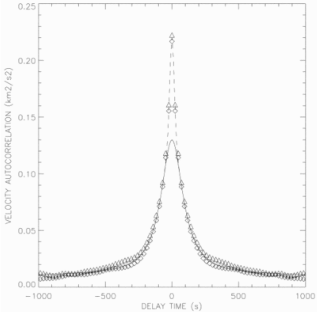
Fig. 3. from Dynamics of Magnetic Flux Elements in the Solar Photosphere van Ballegoijen et al. 1998 ApJ 509 435 doi:10.1086/306471 https://dx.doi.org/10.1086/306471 © 1998. The American Astronomical Society. All rights reserved. Printed in U.S.A.
