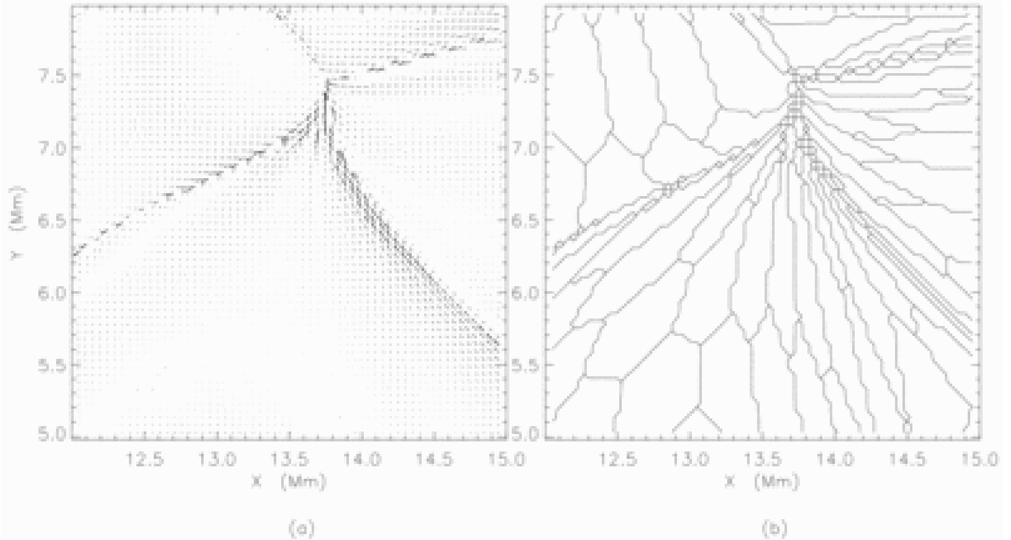
Fig. 10. from Dynamics of Magnetic Flux Elements in the Solar Photosphere van Ballegoijen et al. 1998 ApJ 509 435 doi:10.1086/306471 https://dx.doi.org/10.1086/306471 © 1998. The American Astronomical Society. All rights reserved. Printed in U.S.A.
