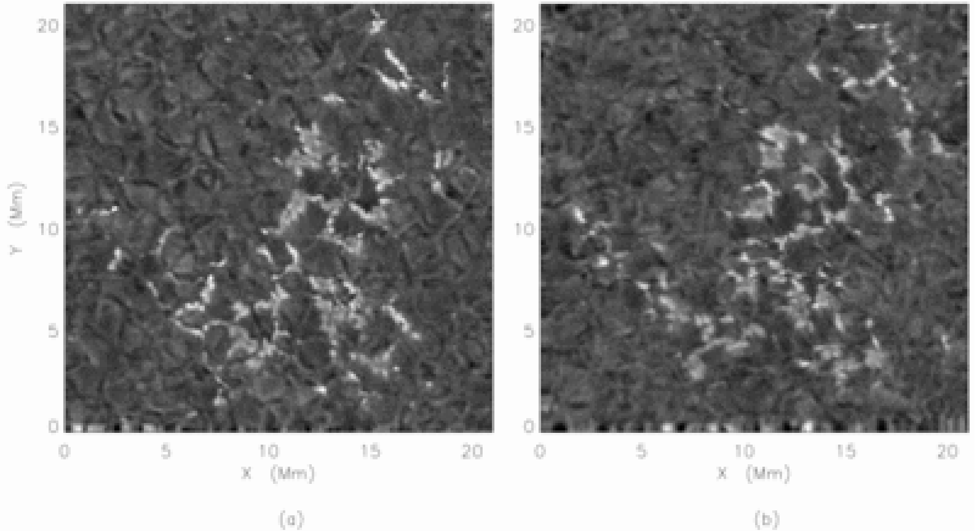
Fig. 1. from Dynamics of Magnetic Flux Elements in the Solar Photosphere van Ballegoijen et al. 1998 ApJ 509 435 doi:10.1086/306471 https://dx.doi.org/10.1086/306471 © 1998. The American Astronomical Society. All rights reserved. Printed in U.S.A.
