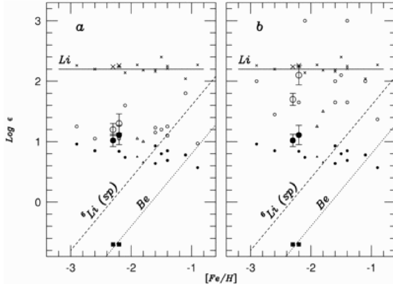
Fig. 9. from Isotopic Lithium Abundances in Nine Halo Stars Smith, Lambert, & Nissen 1998 ApJ 506 405 doi:10.1086/306238 https://dx.doi.org/10.1086/306238 © 1998. The American Astronomical Society. All rights reserved. Printed in U.S.A.
