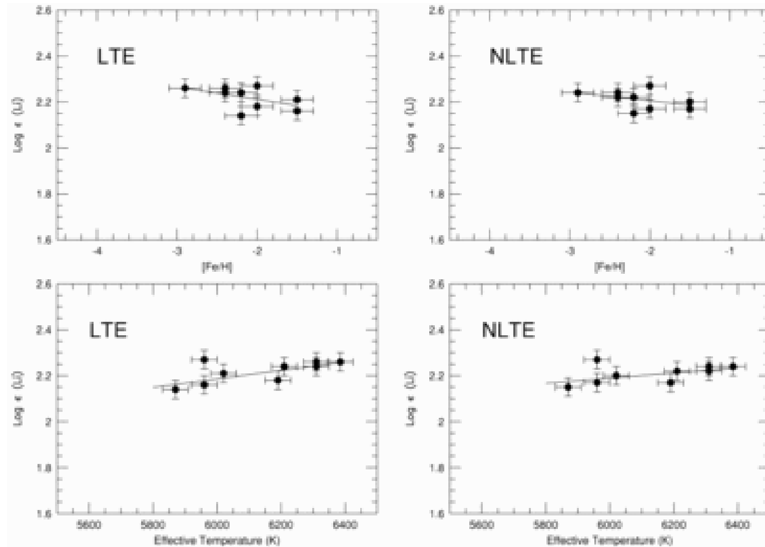
Fig. 8. from Isotopic Lithium Abundances in Nine Halo Stars Smith, Lambert, & Nissen 1998 ApJ 506 405 doi:10.1086/306238 https://dx.doi.org/10.1086/306238 © 1998. The American Astronomical Society. All rights reserved. Printed in U.S.A.
