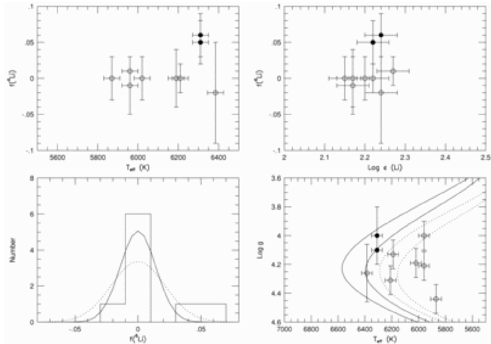
Fig. 7. from Isotopic Lithium Abundances in Nine Halo Stars Smith, Lambert, & Nissen 1998 ApJ 506 405 doi:10.1086/306238 https://dx.doi.org/10.1086/306238 © 1998. The American Astronomical Society. All rights reserved. Printed in U.S.A.
