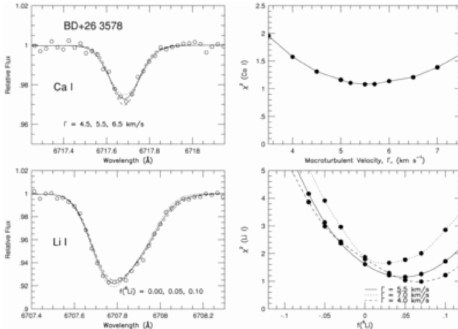
Fig. 6. from Isotopic Lithium Abundances in Nine Halo Stars Smith, Lambert, & Nissen 1998 ApJ 506 405 doi:10.1086/306238 https://dx.doi.org/10.1086/306238 © 1998. The American Astronomical Society. All rights reserved. Printed in U.S.A.
