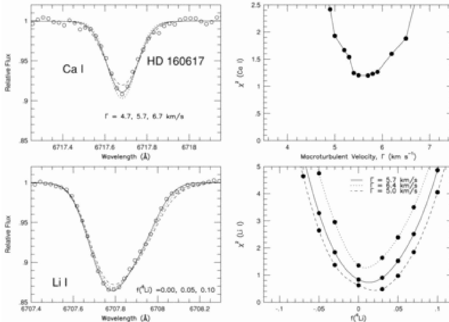
Fig. 5. from Isotopic Lithium Abundances in Nine Halo Stars Smith, Lambert, & Nissen 1998 ApJ 506 405 doi:10.1086/306238 https://dx.doi.org/10.1086/306238 © 1998. The American Astronomical Society. All rights reserved. Printed in U.S.A.
