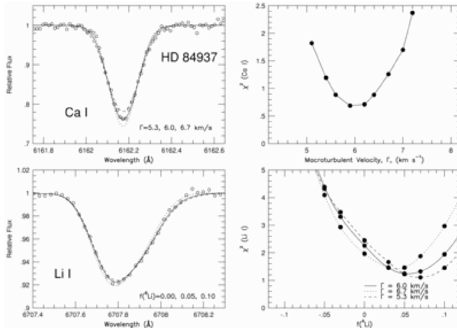
Fig. 4. from Isotopic Lithium Abundances in Nine Halo Stars Smith, Lambert, & Nissen 1998 ApJ 506 405 doi:10.1086/306238 https://dx.doi.org/10.1086/306238 © 1998. The American Astronomical Society. All rights reserved. Printed in U.S.A.
