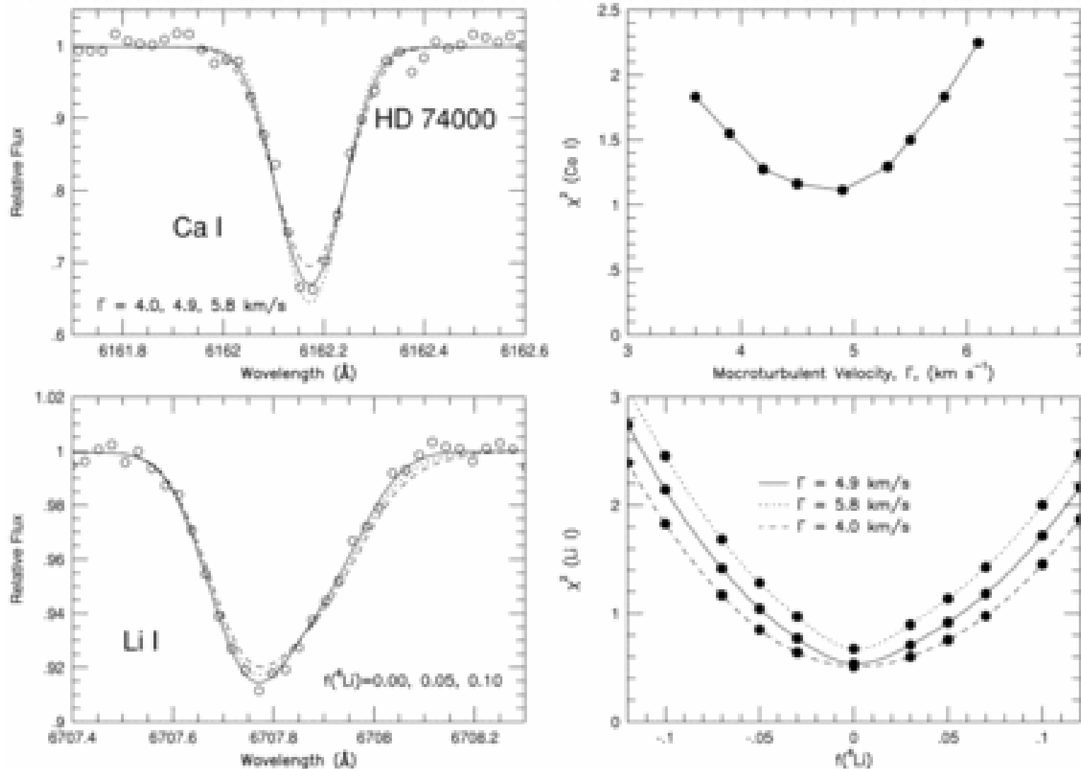
Fig. 3. from Isotopic Lithium Abundances in Nine Halo Stars Smith, Lambert, & Nissen 1998 ApJ 506 405 doi:10.1086/306238 https://dx.doi.org/10.1086/306238 © 1998. The American Astronomical Society. All rights reserved. Printed in U.S.A.
