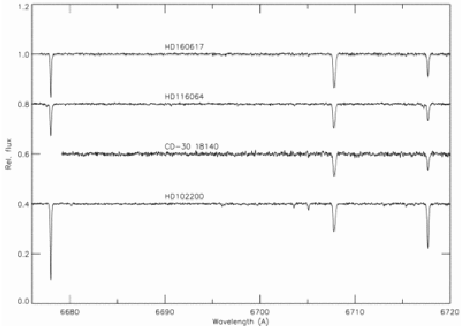
Fig. 2. from Isotopic Lithium Abundances in Nine Halo Stars Smith, Lambert, & Nissen 1998 ApJ 506 405 doi:10.1086/306238 https://dx.doi.org/10.1086/306238 © 1998. The American Astronomical Society. All rights reserved. Printed in U.S.A.
